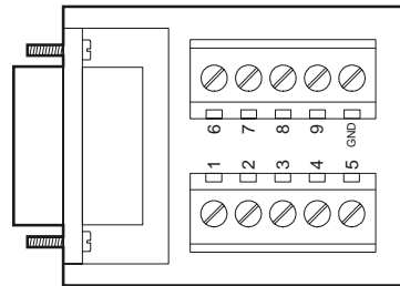
Figure 6 - Pin Configuration for Accessories PCB
