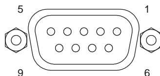
Figure 5 - DB-9 Pin Configuration For RS-232 Serial Port
