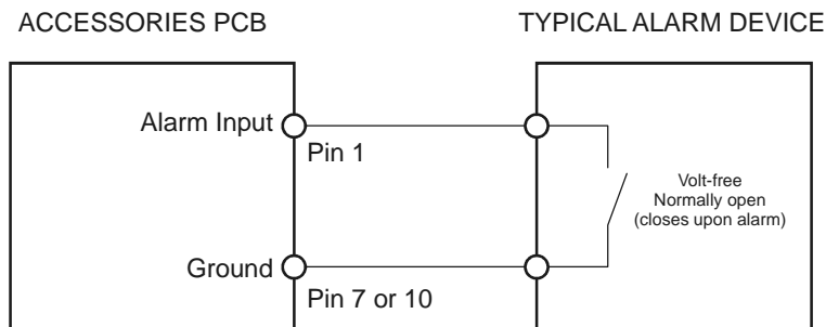
Figure 7 - A Normally Open Relay Alarm Condition
