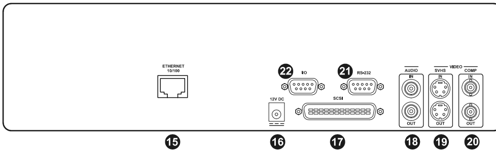
Figure 3 - Rear Panel Connections
