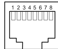
Figure 4 - RJ-45 Pin Configuration For Ethernet Port
